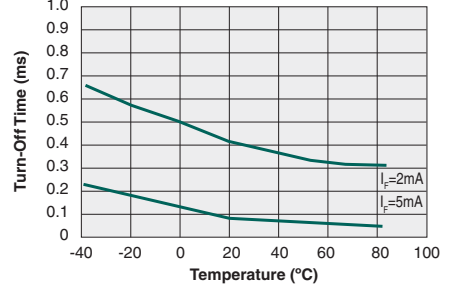
Typical Turn-Off Time vs. Temperature ( I_F=120mA_{DC} )
