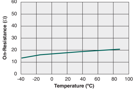
Typical On-Resistance vs. Temperature ( I_F=2mA , I_L=120mA_{DC} )
