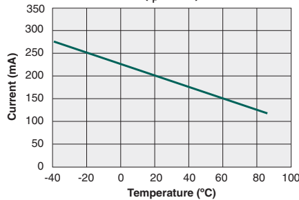
Typical Current Limiting vs. Temperature ( I_F=2mA )
